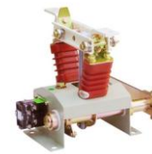
7.2kV 1P 200~600A Insulating class : 6A(60BIL) Rated Short-time with stand current : 25kA / 1sec Auxiliary contacts : 2a2b~10a10b Automatic, Manual
