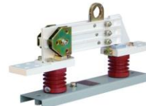
7.2kV 1P 1600~2000A Insulating class : 6A(60BIL) Rated Short-time with stand current : 25kA / 1sec Auxiliary contacts : - Hook
